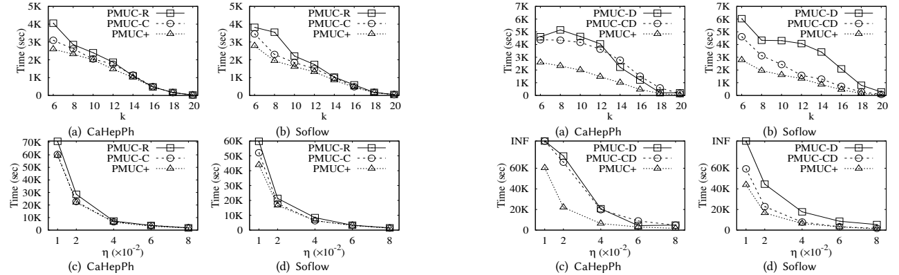
Figure 4: Runtime of pivot-based algorithms with different ordering techniques
