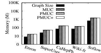
Figure 10: Memory usages of different algorithms
