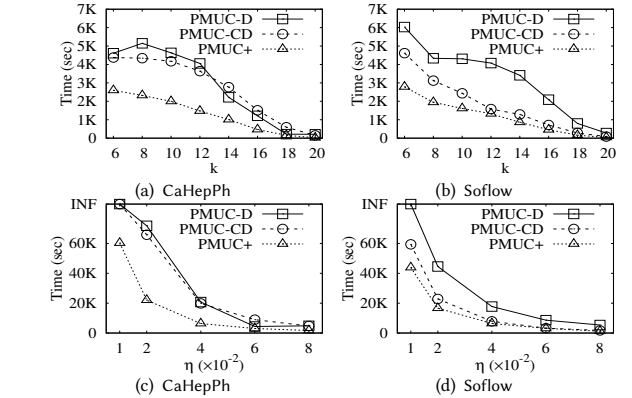
Figure 5: Runtime of pivot-based algorithms with different pivot selection strategies
